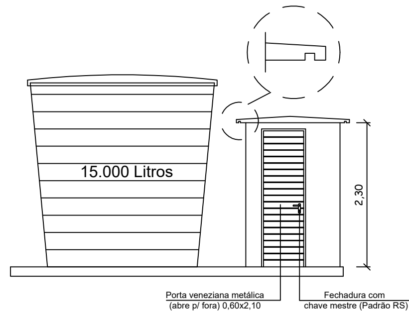
Vista Frontal
